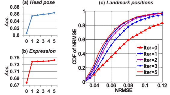
Figure 4: Iterative performance improvement for each task on the 300-W evaluation set.
