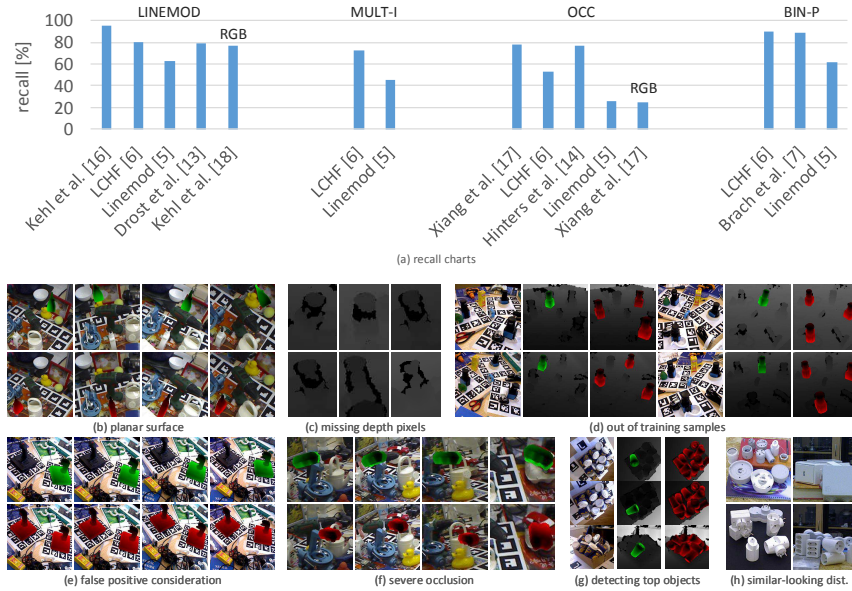
Fig. 2: (a) Success of each baseline on every dataset is shown, recall values are computed using the Average Distance (AD) metric. (b)-(h) challenges encountered during test are exemplified (green renderings are hypotheses, and the red ones are ground truths).
